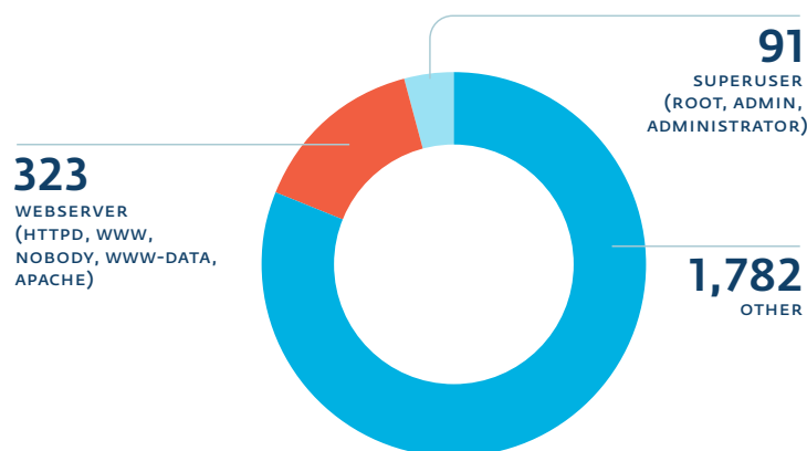
Figure 3.19 Numbers of Unique Infections
