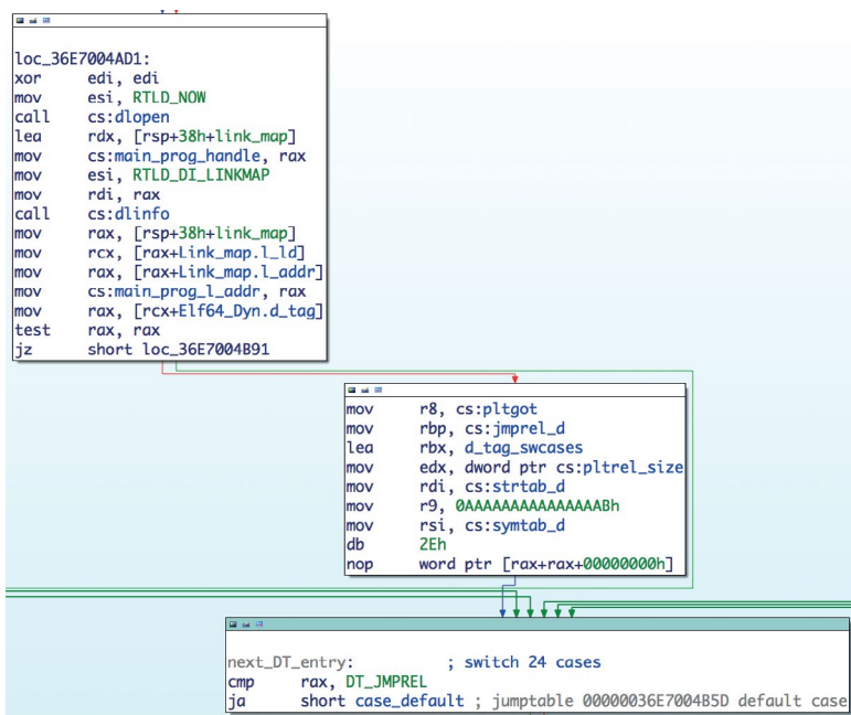
Figure 4.2 Parsing original executable ELF headers in libkeyutils.so
