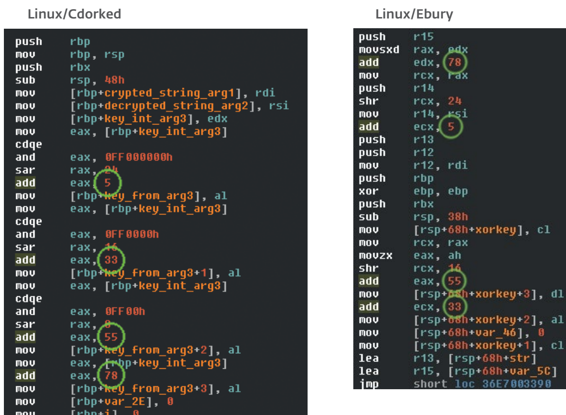
Figure 3.3 Comparing Linux/Cdorked and Linux/Ebury custom cryptography
