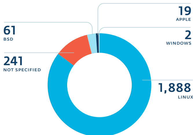
Figure 3.18 Perl/Calfbot username distribution
