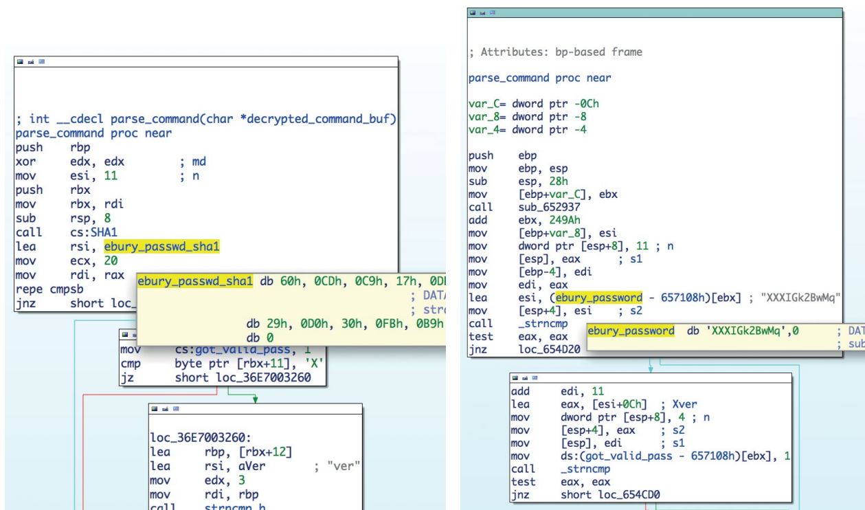
Figure 4.1 Linux/Ebury access password now hashed
