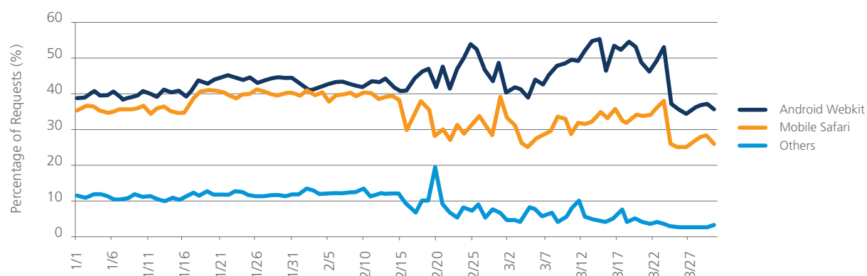
Figure 32: Mobile Browsers Seen Across Cellular Networks, Q1 2013
