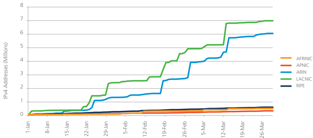
Figure 8: Total Number of IPv4 Addresses Assigned/Allocated by RIR, Q1 2013
