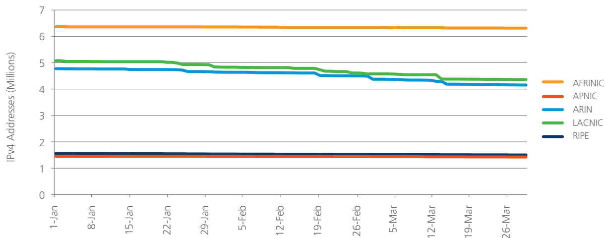
Figure 7: Available IPv4 Address Pool Size by RIR, Q1 2013
