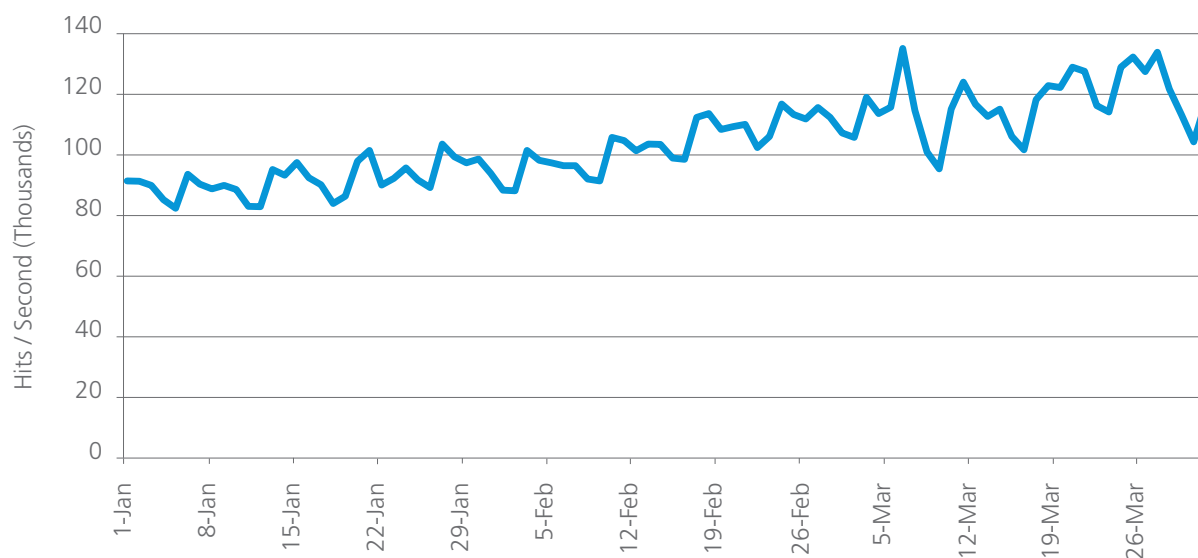
Figure 10: IPv6 Traffic to the Akamai Intelligent Platform, Q1 2013
